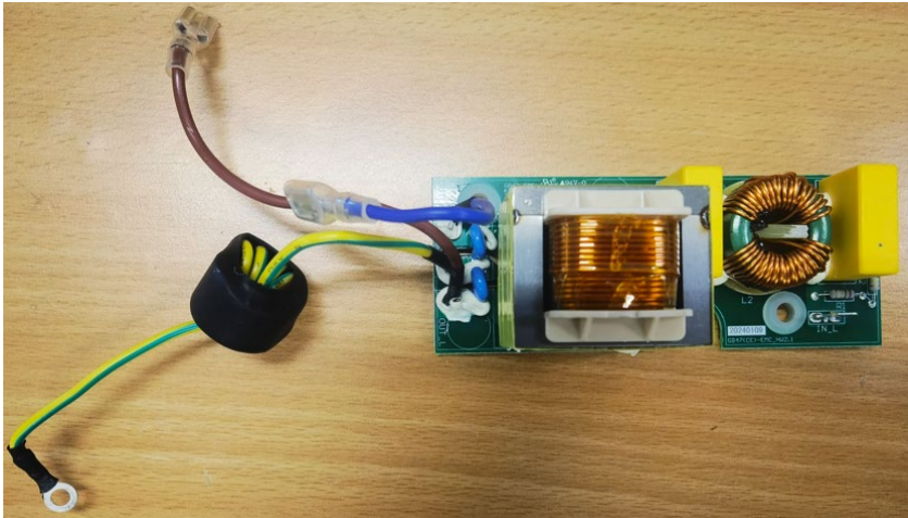
RFI Board, 230 V 990428000
