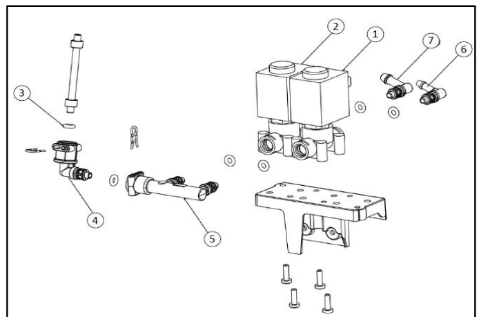
Solenoid valve assembly - steam - 968956
