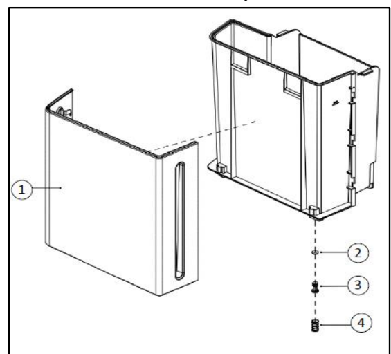
Watertank 6L assembly - 968864
