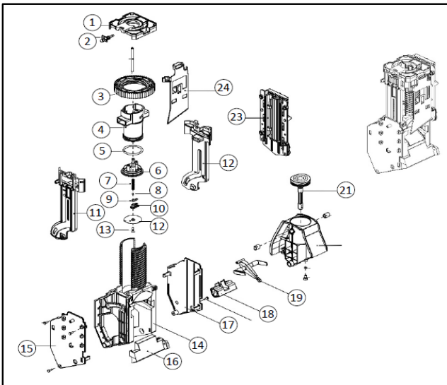
Brew unit assembly - 968895
