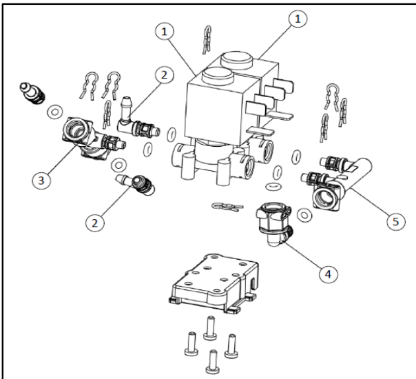
Solenoid valve assembly - Hot water - 968949
