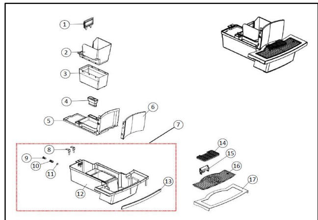
Drip tray assembly - 968871
