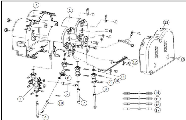
Thermoblock assembly - 968918
