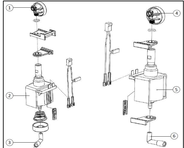
Pump A assembly - 969007 Pump B assembly - 969014
