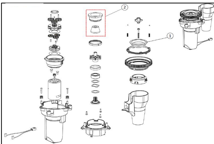
Grinder group assembly - 968888
